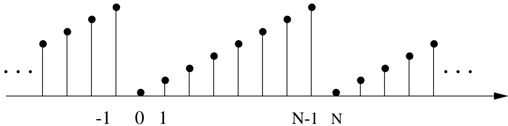
Fig. 3.3. A Wavelet Tour of Signal Processing, 3 rd ed. Signal f[n] = n for 0 \leq n < N made periodic over N samples.
