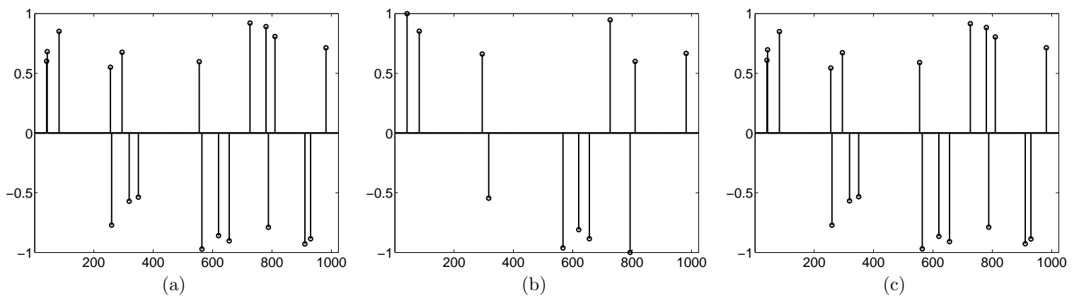
Fig. 13.9. A Wavelet Tour of Signal Processing, 3 rd ed. (a): Sparse spike f . (b) Estimation \tilde{F}_1 from Y = u_1 \star f + W . (c) Estimation \tilde{F}_2 from Y = u_2 \star f + W .
