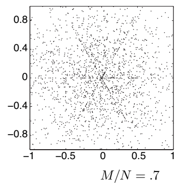
Fig. 13.12. A Wavelet Tour of Signal Processing, 3 rd ed. Distribution of synthetic coefficients \{\vec{b}[p]\}_p computed with S = 3 sources having M non-zero coefficients randomly distributed among the N coordinates of a basis.
