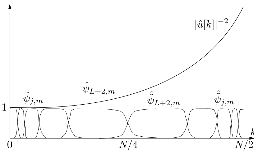
Fig. 13.1. A Wavelet Tour of Signal Processing, 3 rd ed. The singular spectrum |\hat{u}[k]|^2 of a low-pass filter decreases to zero at high frequencies. The relative variation of |\hat{u}[k]|^{-2} is not large over the frequency support of each wavelet and mirror wavelet of a mirror wavelet basis.
