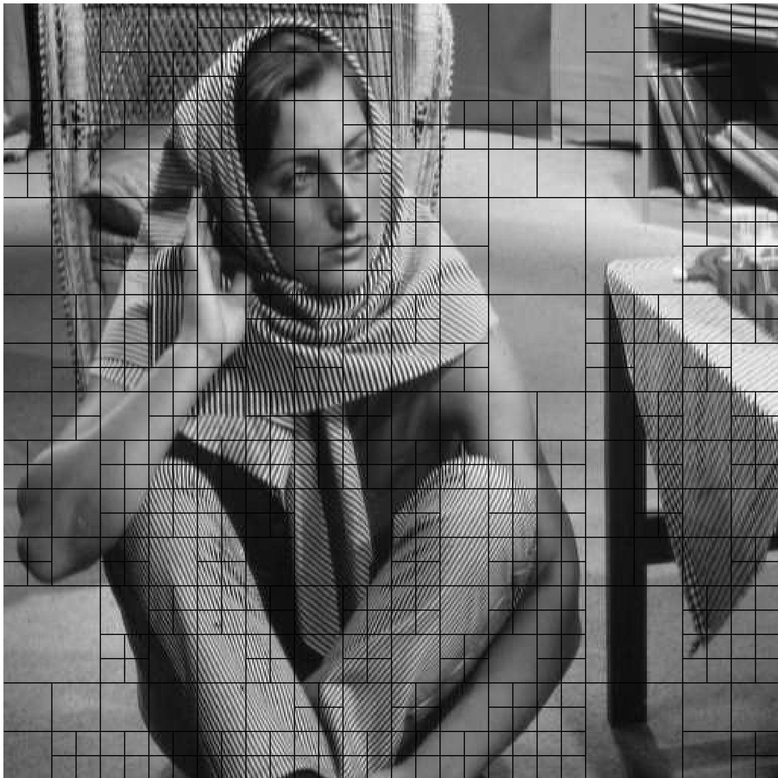
Fig. 12.5. A Wavelet Tour of Signal Processing, 3 rd ed. The grid shows the approximate support of square overlapping windows in the best local cosine basis, computed with an \mathbf{l}^1 cost.
