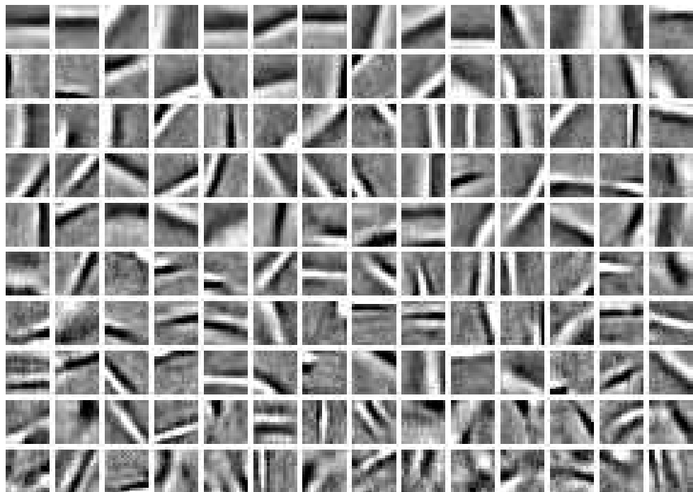
Fig. 12.25. A Wavelet Tour of Signal Processing, 3 rd ed. Some vectors \phi_p of a dictionary \mathcal{D} learned from a set of patches extracted from natural images.
