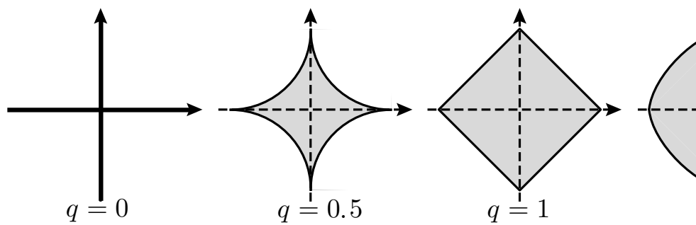
Fig. 12.22. A Wavelet Tour of Signal Processing, 3 rd ed. Unit balls for the L^q functionals.
