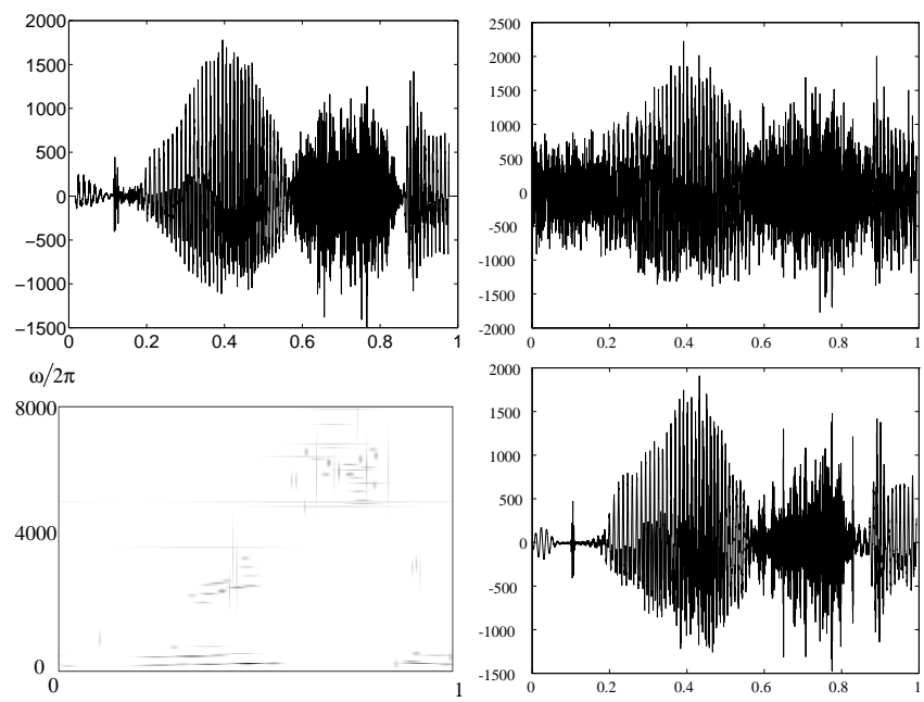
Fig. 12.18. A Wavelet Tour of Signal Processing, 3 rd ed. (a): Speech recording of “greasy.” (b): Recording of “greasy” plus a Gaussian white noise (SNR = 1.5 db). (c): Time-frequency distribution of the M = 76 coherent Gabor structures. (d): Estimation \hat{F} reconstructed from the 76 coherent structures (SNR = 6.8 db).
