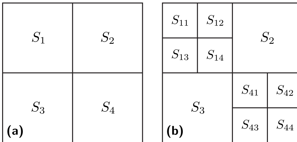
Fig. 12.10. A Wavelet Tour of Signal Processing, 3 rd ed. (a-c) Construction of a dyadic segmentation by successive subdivisions. (d) Quadtree representation of the segmentation. Each leaf of the tree indicates a square in the segmentation and can be represented with a binary string whose length is proportional to the depth of the tree.
