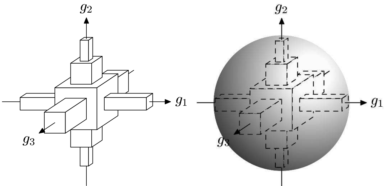
Fig. 11.10. A Wavelet Tour of Signal Processing, 3 rd ed. (a): Example of orthosymmetric set \Theta in three dimensions. (b): The quadratically convex hull QH[\Theta] is a larger ellipsoid including \Theta .
