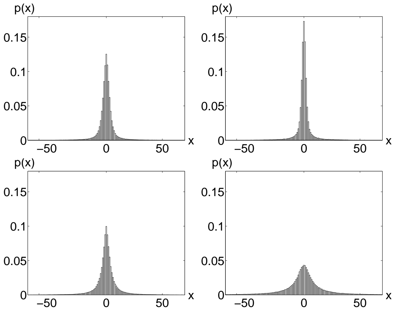
Fig. 10.9. A Wavelet Tour of Signal Processing, 3 rd ed. Normalized histograms of orthogonal wavelet coefficients for each image.
