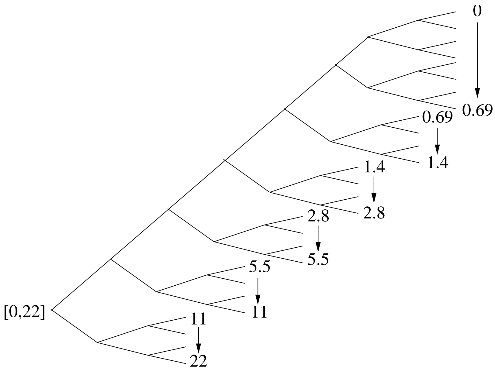
Fig. 10.5. A Wavelet Tour of Signal Processing, 3 rd ed. Wavelet packet tree that decomposes the frequency interval [0, 22\text{kHz}] in 24 frequency bands covered by M = 4 wavelets dilated over six octaves, plus eight low frequency bands of the same bandwidth. The frequency bands are indicated at the leaves in kHz.
