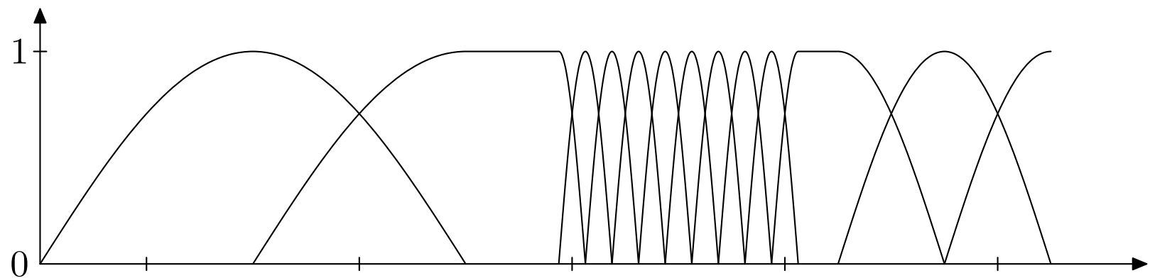
Fig. 10.4. A Wavelet Tour of Signal Processing, 3 rd ed. Succession of windows of various sizes on intervals of 2048 samples, which satisfy the orthogonality constraints of local cosine bases.
