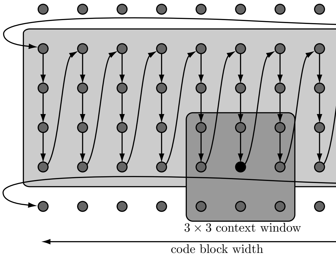
Fig. 10.17. A Wavelet Tour of Signal Processing, 3 rd ed. JPEG-2000 scans square blocks of L \times L wavelet coefficients, as bands of size 4 \times L .
