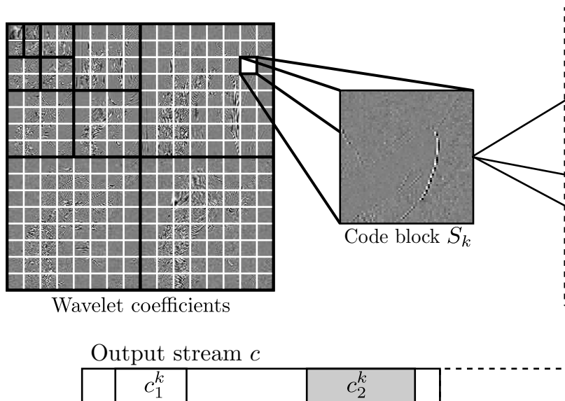
Fig. 10.16. A Wavelet Tour of Signal Processing, 3 rd ed. Overview of JPEG-2000 compression process.
