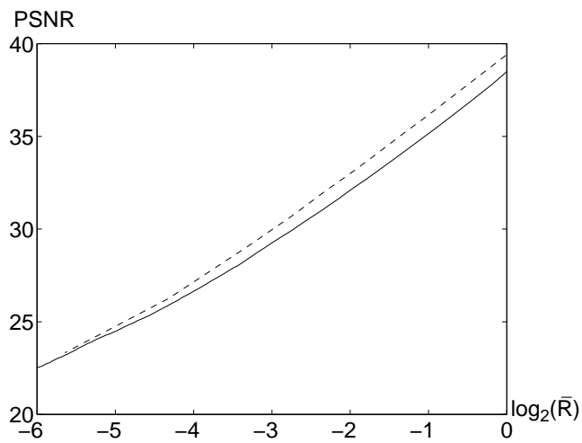
Fig. 10.12. A Wavelet Tour of Signal Processing, 3 rd ed. Comparison of the PSNR obtained with an embedded wavelet transform code (dotted line) and a direct wavelet transform code (solid line)
