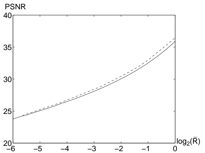
Fig. 10.12. A Wavelet Tour of Signal Processing, 3 rd ed. Comparison of the PSNR obtained with an embedded wavelet transform code (dotted line) and a direct wavelet transform code (solid line)
