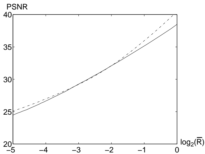
Fig. 10.11. A Wavelet Tour of Signal Processing, 3 rd ed. PSNR as a function of \log_2(\bar{R}) . (a) Lena (solid line) and boats (dotted line) (b) Goldhill (solid line) and Mandrill (dotted line)
