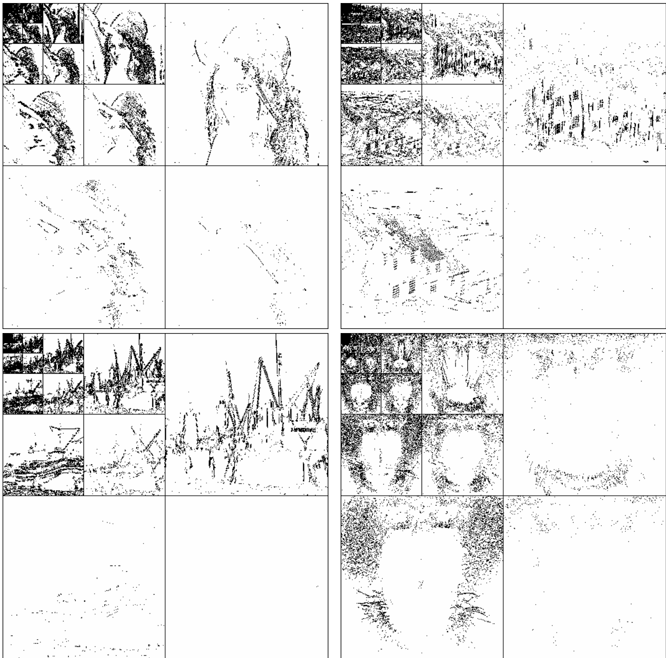
Fig. 10.10. A Wavelet Tour of Signal Processing, 3 rd ed. Significance maps of quantized wavelet coefficients for images coded with \bar{R} = 0.5 bit/pixel.
