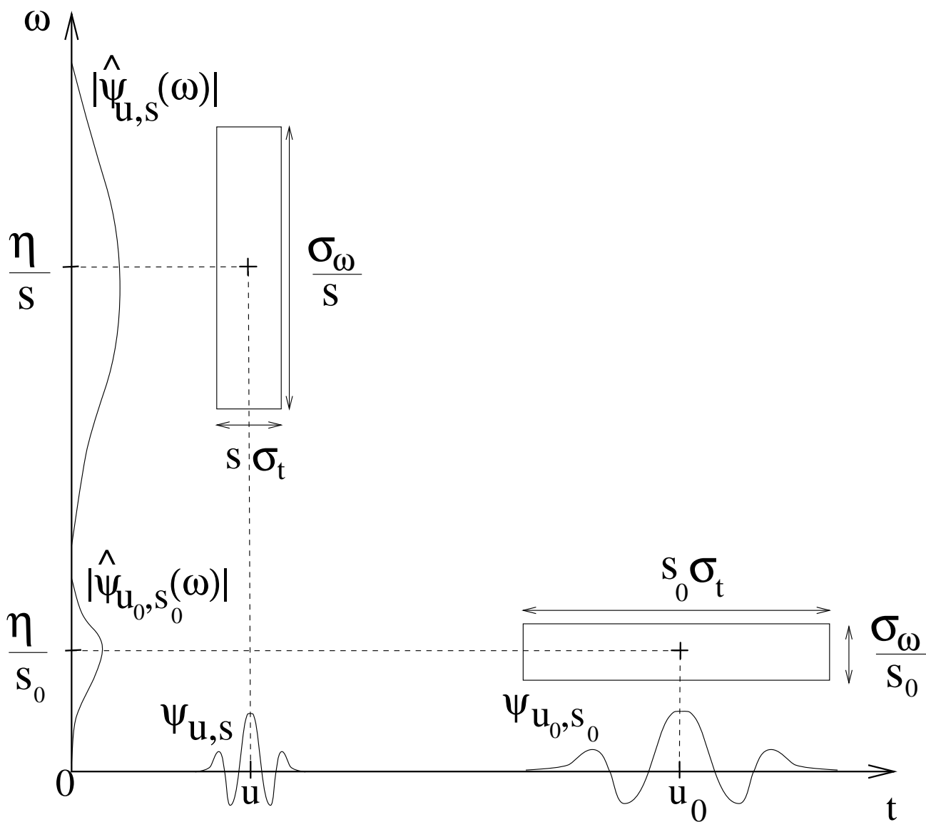
Fig. 1.5. A Wavelet Tour of Signal Processing, 3 rd ed. Heisenberg time-frequency boxes of two wavelets \psi_{u,s} and \psi_{u_0,s_0} . When the scale s decreases, the time support is reduced but the frequency spread increases and covers an interval that is shifted towards high frequencies.
