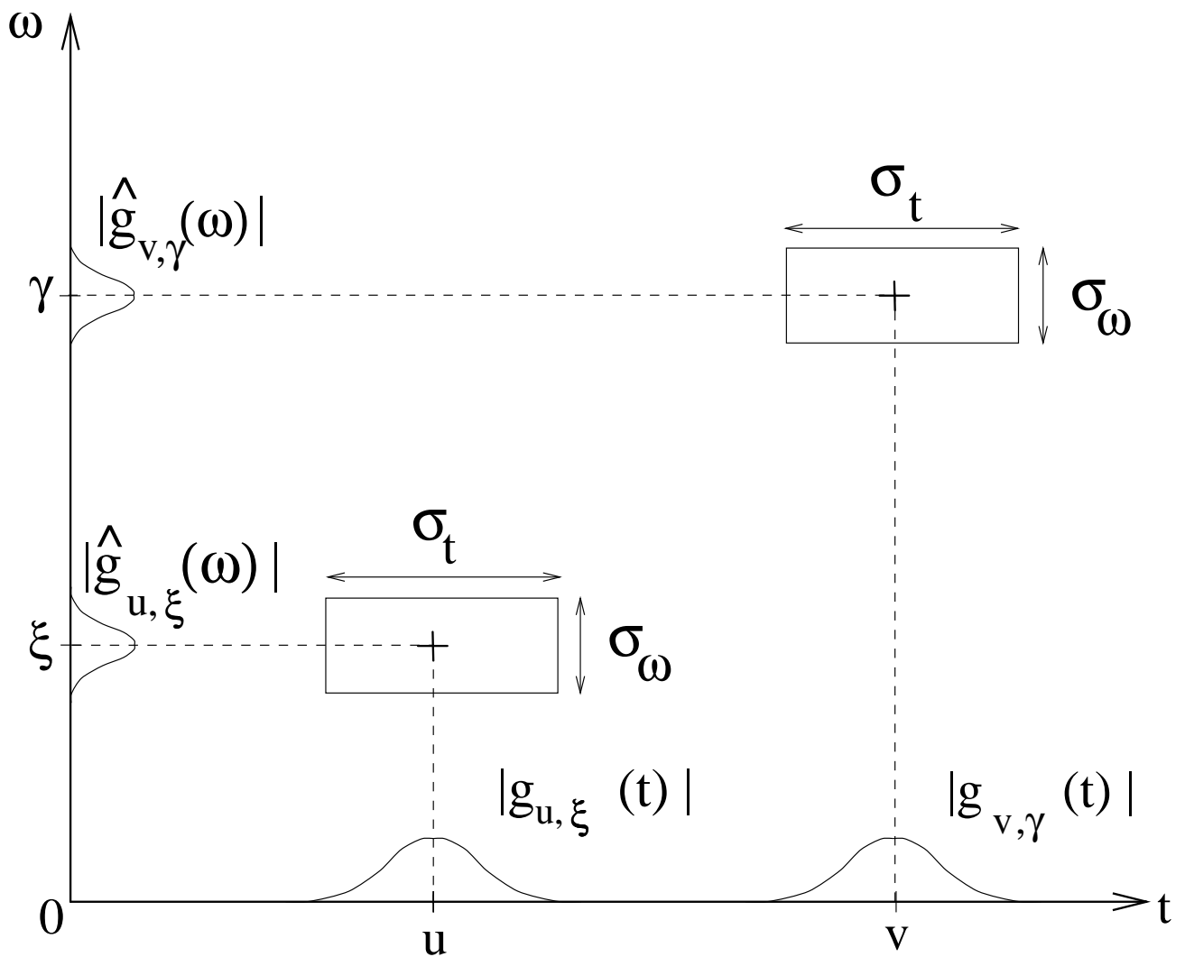
Fig. 1.4. A Wavelet Tour of Signal Processing, 3 rd ed. Time-frequency boxes (“Heisenberg rectangles”) representing the energy spread of two windowed Fourier atoms.
